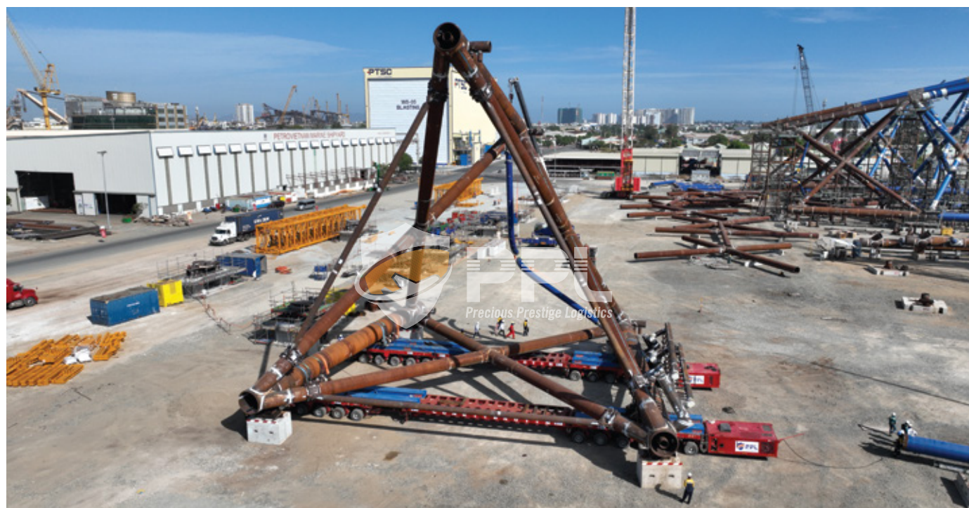
Upper Jacket (UJ) 27 x 24 x 24 m 325.7 tons
